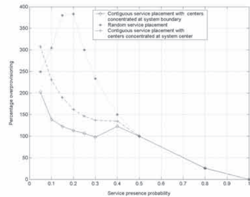
Figure 12: Amount of over-provisioning due to overlapping SFN areas
