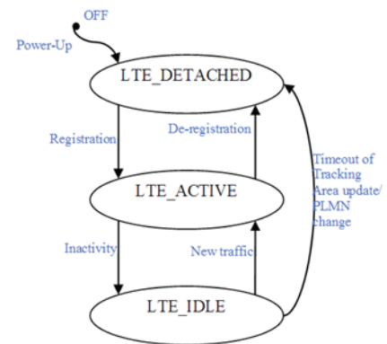
Figure 9: Mobility states of the UE in LTE.
