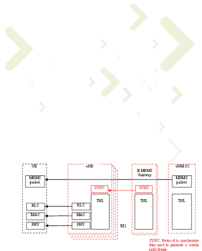
Figure 10: The overall U-plane architecture of the MBMS content synchronization [4]
