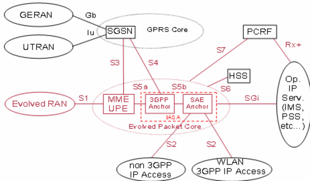
Figure 15 System architecture evolution
