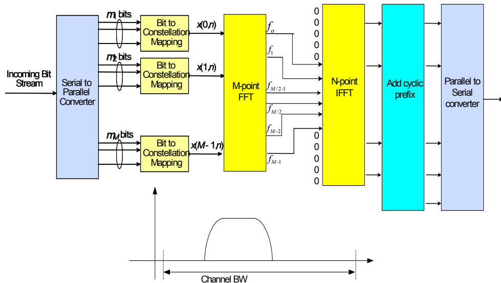
Figure 8 Block Diagram of DFT-s-OFDM (Localized transmission)
