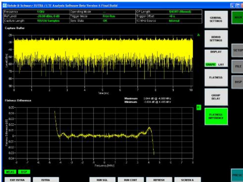
Figure 27 Measurement of flatness difference
