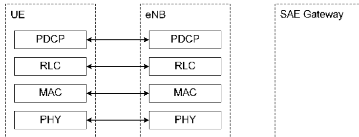
Figure 17 User plane protocol stack
