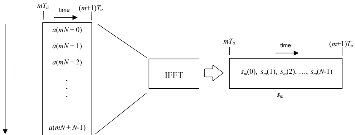
Figure 2 OFDM Useful Symbol Generation using an IFFT
