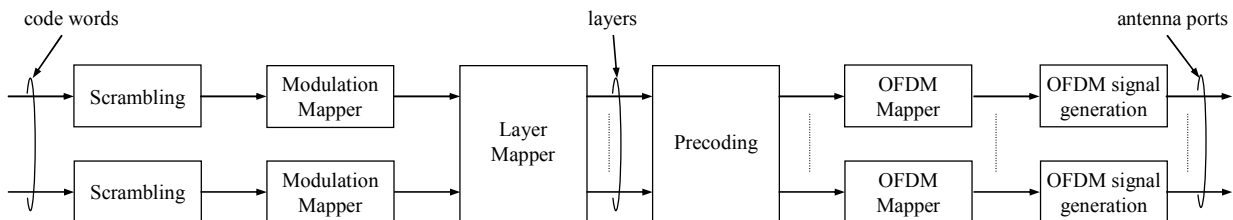
Figure 14 Overview of downlink baseband signal generation
