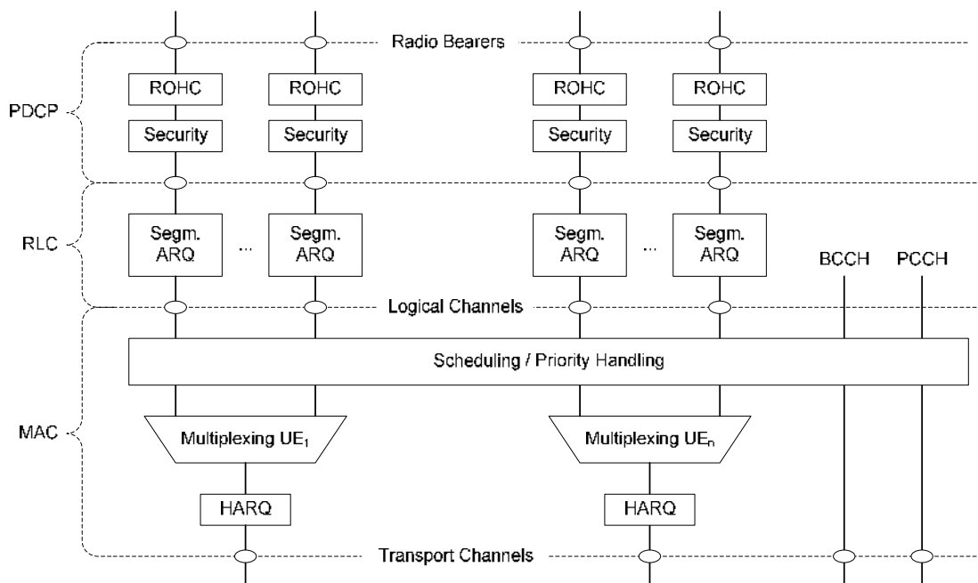
Figure 19 Downlink layer 2 structure
