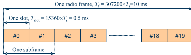
Figure 4 Generic frame structure in E-UTRA downlink
