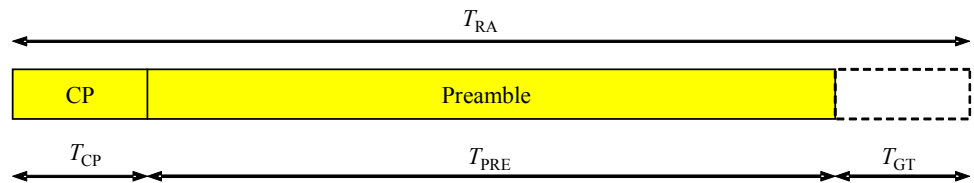
Figure 11 Random access preamble
