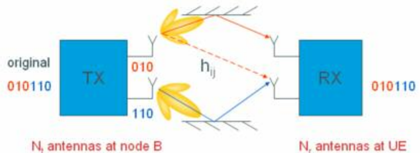
Figure 12 Spatial multiplexing
