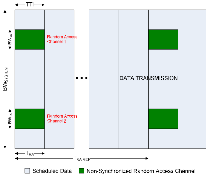
Figure 10 Random access structure, principle
