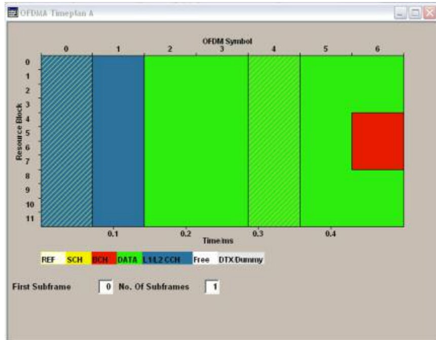
Figure 23 OFDMA time plan for LTE signal generation, 1 slot
