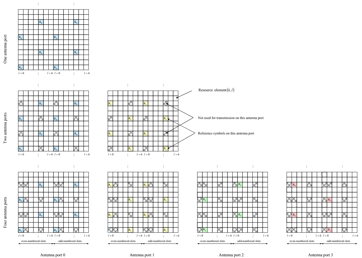
Figure 6 Downlink reference signal structure (normal cyclic prefix)
