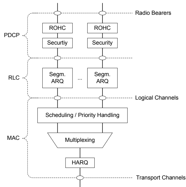
Figure 20 Uplink layer 2 structure
