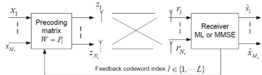
Figure 13 Precoding principle
