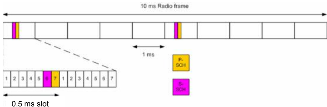
Figure 7 P-SCH and S-SCH structure
