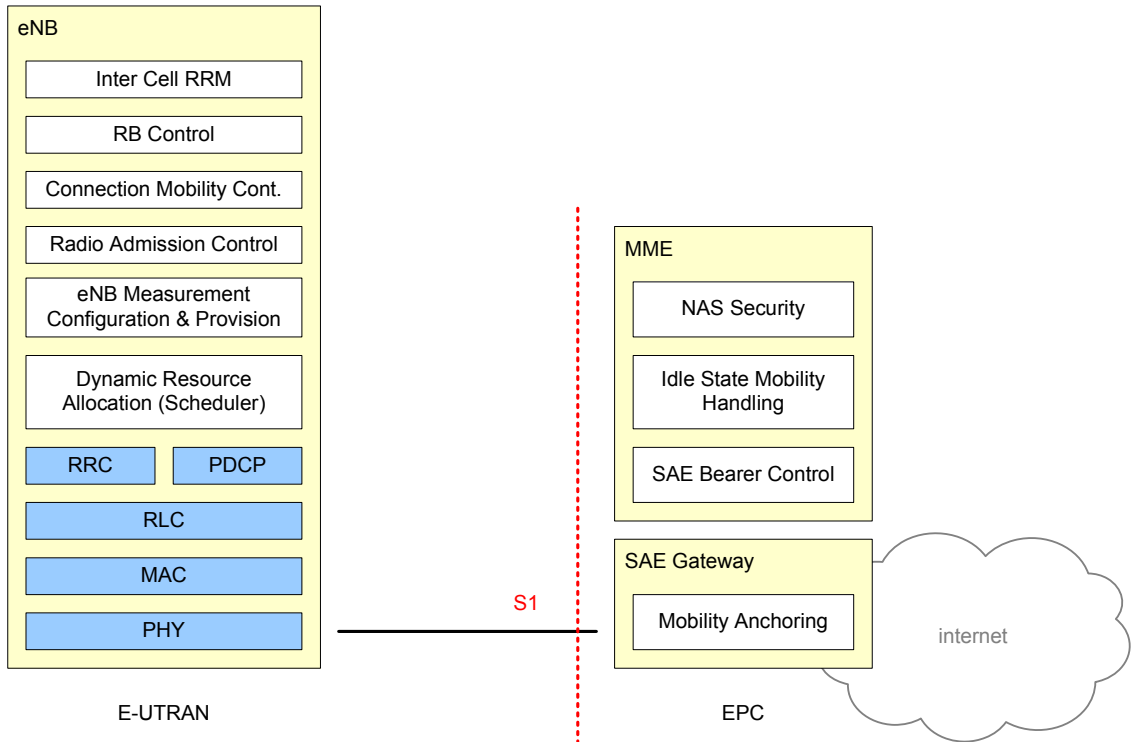
Figure 16 Functional split between E-UTRAN and Evolved Packet Core
