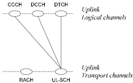
Figure 22 Mapping between uplink logical and transport channels
