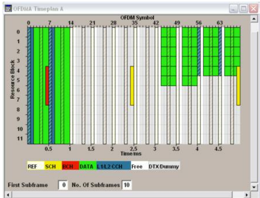
Figure 24 OFDMA time plan for LTE signal generation, 10 slots
