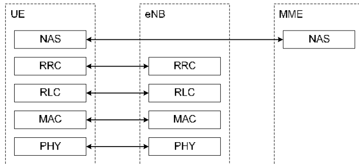
Figure 18 Control plane protocol stack
