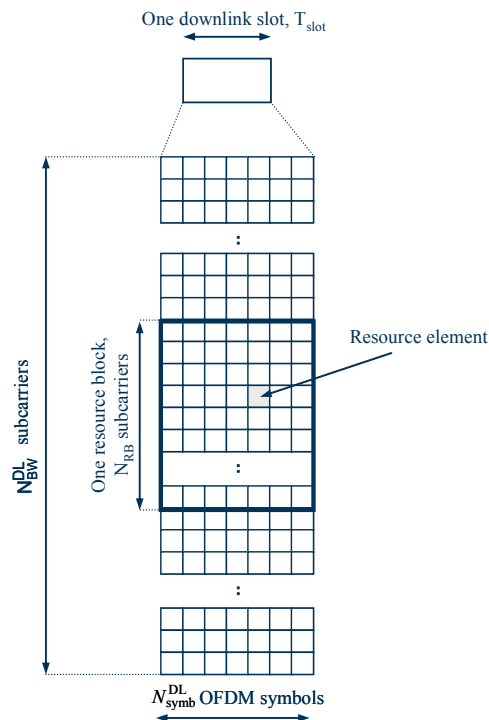
Figure 5 Downlink resource grid
