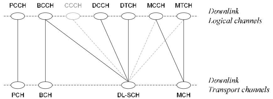
Figure 21 Mapping between downlink logical and transport channels
