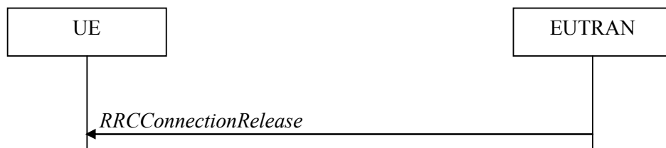
Figure 2: RRC connection release procedure [8]
