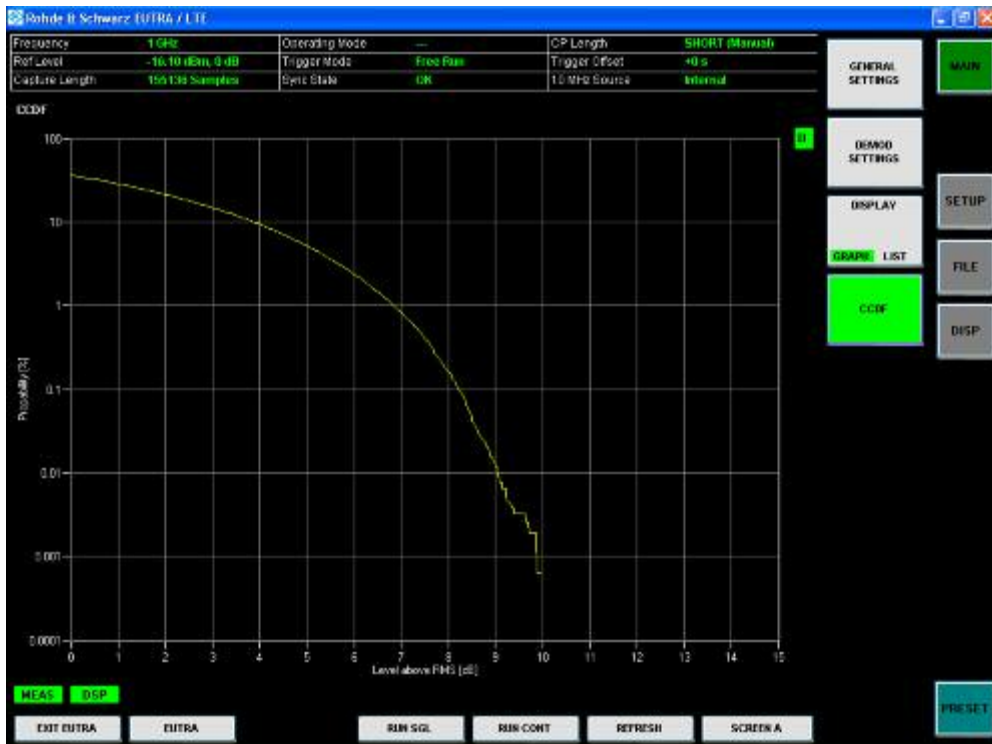
Figure 26 CCDF measurement
